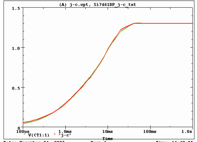
Si7461DP Tank j-c Temperature: 27.0
