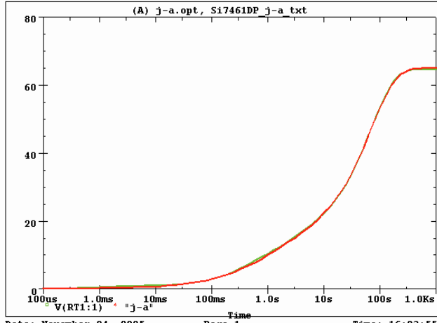
Si7461DP Tank j-a Temperature: 27.0
