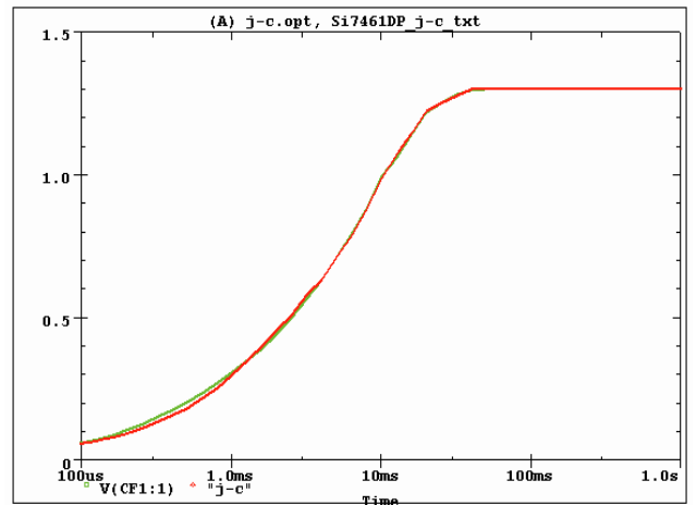
Si7461DP Filter j-c Temperature: 27.0
