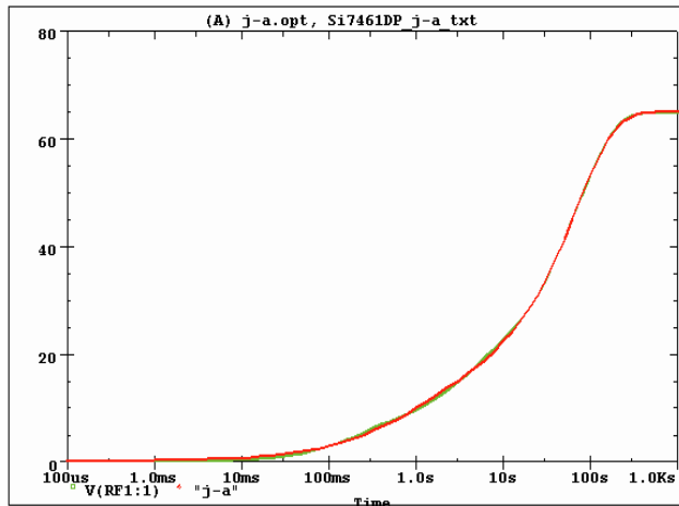
Si7461DP Filter j-a Temperature: 27.0
